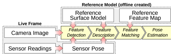
Figure 5: Flowchart of the proposed camera localization framework for outdoor environments.
